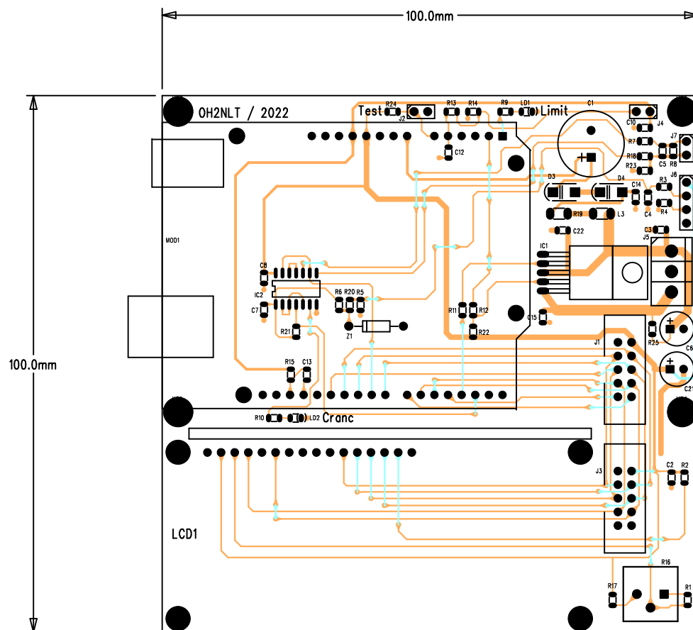
RevCtr Main board Rev V2.0 25.2.2022
